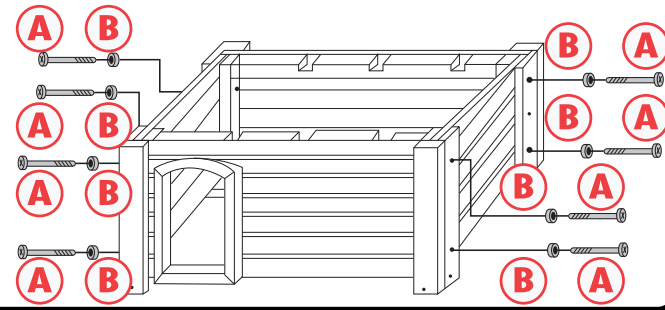
Side Panel
